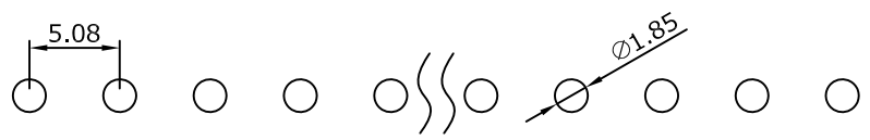
Recommended PCB Layout (PCB TOLERANCE ±0.05)
