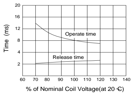
Operate time/Release time
