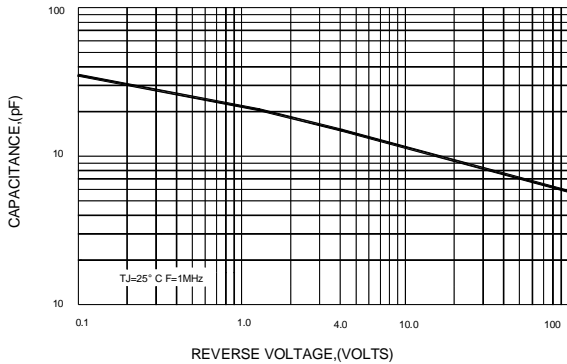
FIG.5-TYPICAL JUNCTION CAPACITANCE
